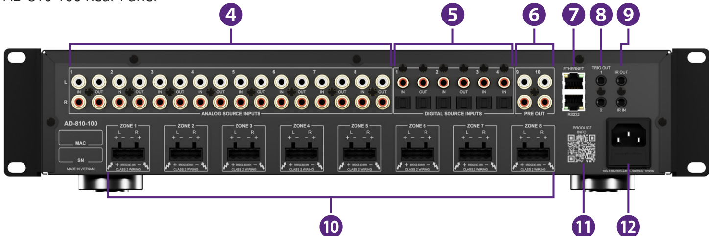
AD-810-100 Rear Panel
