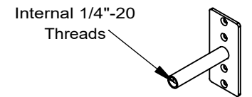
DETAIL R SCALE 1 : 5
