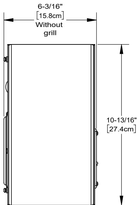
Right view
