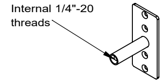
DETAIL A SCALE 1 : 4
