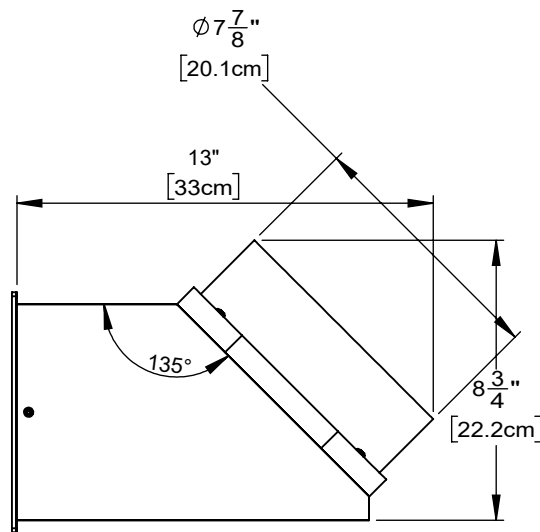
Right view
