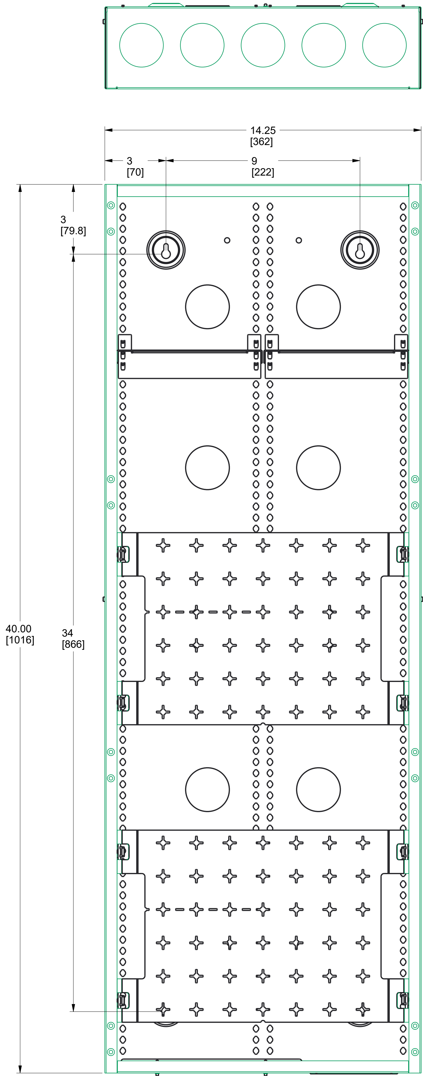
WIREFATH ONE,40IN, TOP ASSY
