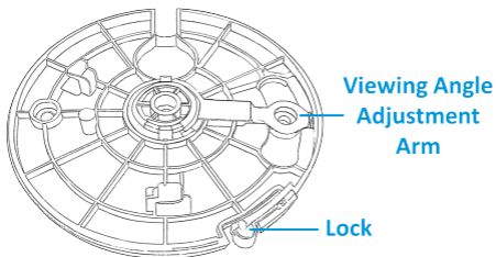
Mounting Plate
