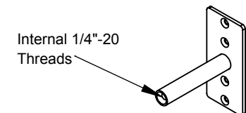
DETAIL P SCALE 1 : 4
